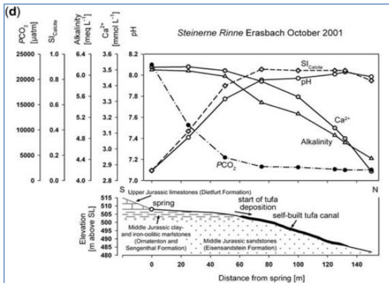
Figure 2.4: An example of the downstream changes in CO 2 pressure (pCO 2 ) calcite saturation (SI calcite ) Alkalinity, Calcium concentration and pH along a stream with travertine deposition (after Arp et al. 2010)
