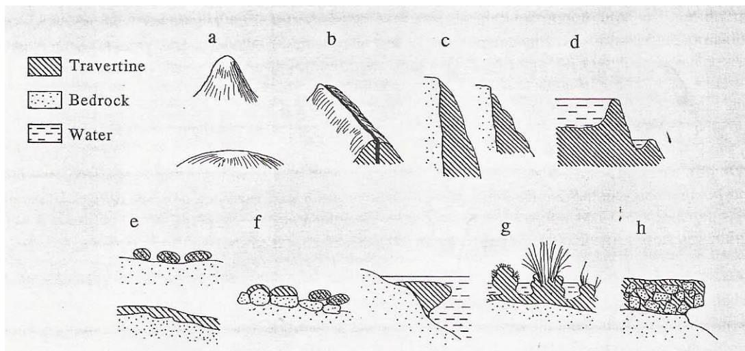
Figure 3.3: Different types of travertine formation (after Pentecost 1995).
