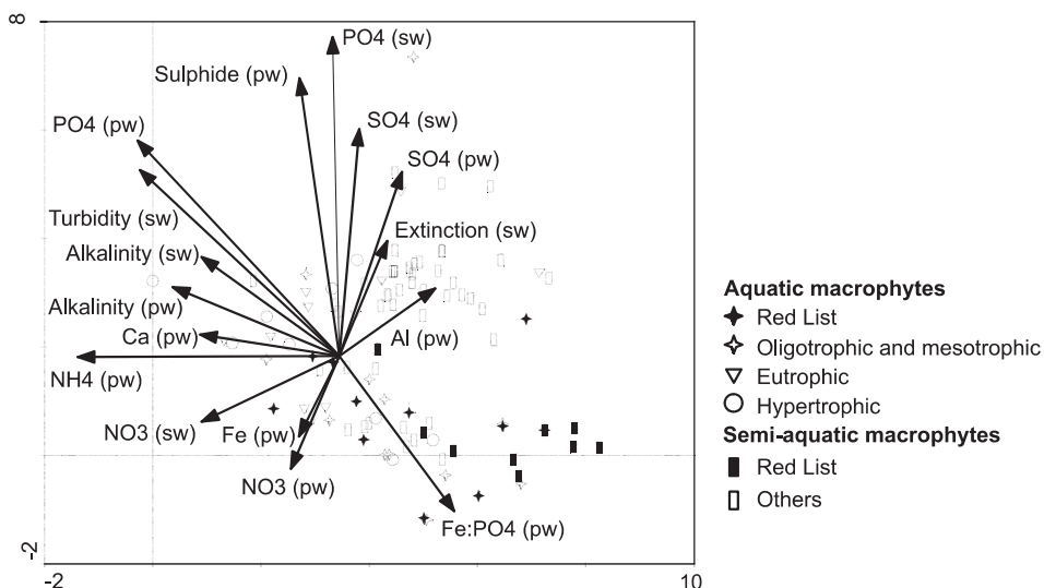
Figure 7. Indirect ordination diagram (DCA) of macrophyte species showing the first two axes (different dots for each category) with environmental variables included (arrows). pw = pore water, sw = surface water.
