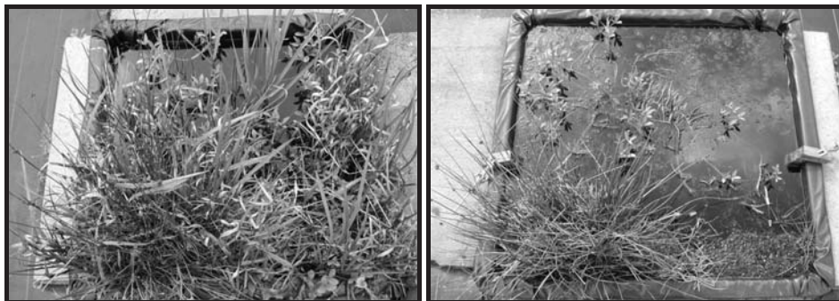
Figure 8. Photographs of two fertilized mesocosms at the end of the third growing season (September 2007) without (left) and with \text{SO}_4 addition (right).
