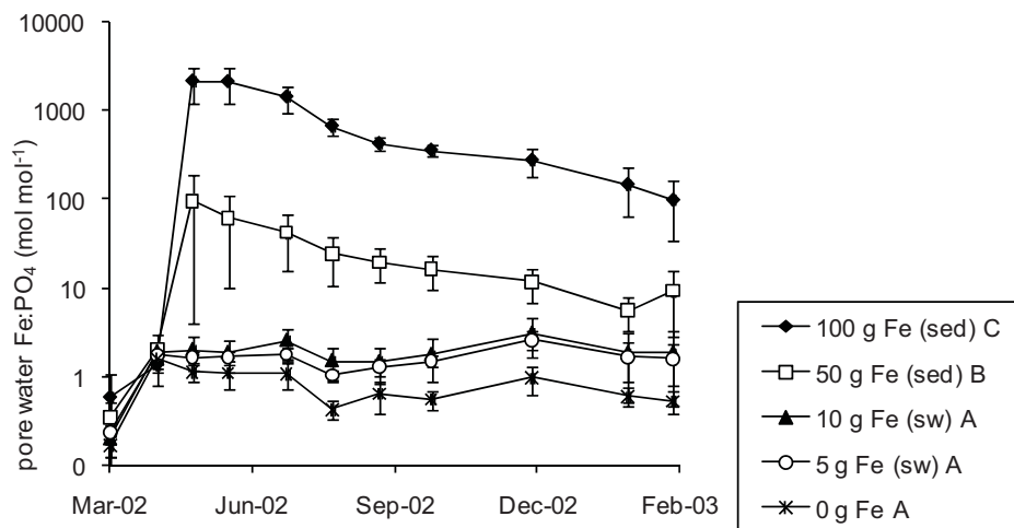
Figure 3. Effects of the various treatments on the Fe: \text{PO}_4 ratio in the sediment pore water ( \pm\text{SEM} ). Treatments started after the second sampling date. Letters indicate differences between treatments ( P < 0.05 ). sw = surface water treatment, sed = sediment treatment. Note the logarithmic y-axis.
