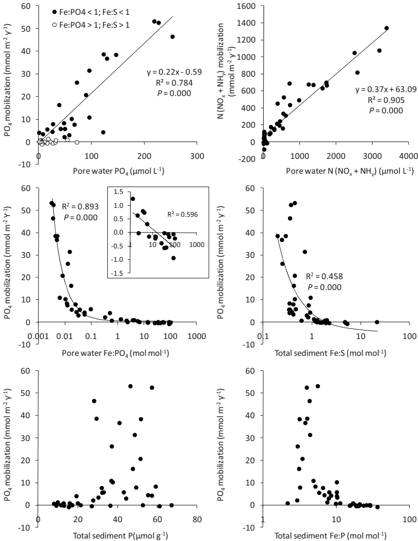
Figure 4. Relationship between sediment and pore water characteristics and mobilization rates of \text{PO}_4 and N ( \text{NO}_x and \text{NH}_y ) from peat sediments to the water layer.
