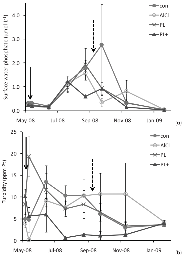
Figure 5. Surface water PO 4 concentrations (a) and turbidity (b) in an enclosure experiment in the Dutch peat lake Tienhovense Plassen (Geurts & Van de Wouw, unpublished data). The following treatments were applied (n=3): con = control, AICI = 40 g m -2 aluminium chloride, PL = 385 g m -2 LMC (Phoslock®), PL+ = 425 g m -2 LMC (Phoslock®) + polyaluminum chloride. The solid arrow indicates the start of the treatments. The dashed arrow indicates PO 4 addition of 10 μmol L -1 . PO 4 concentrations in the PL+ treatment differed significantly from the control ( P = 0.020 ; GLM repeated measures). For turbidity there was a significant time x treatment effect ( P = 0.000 ; GLM repeated measures).
