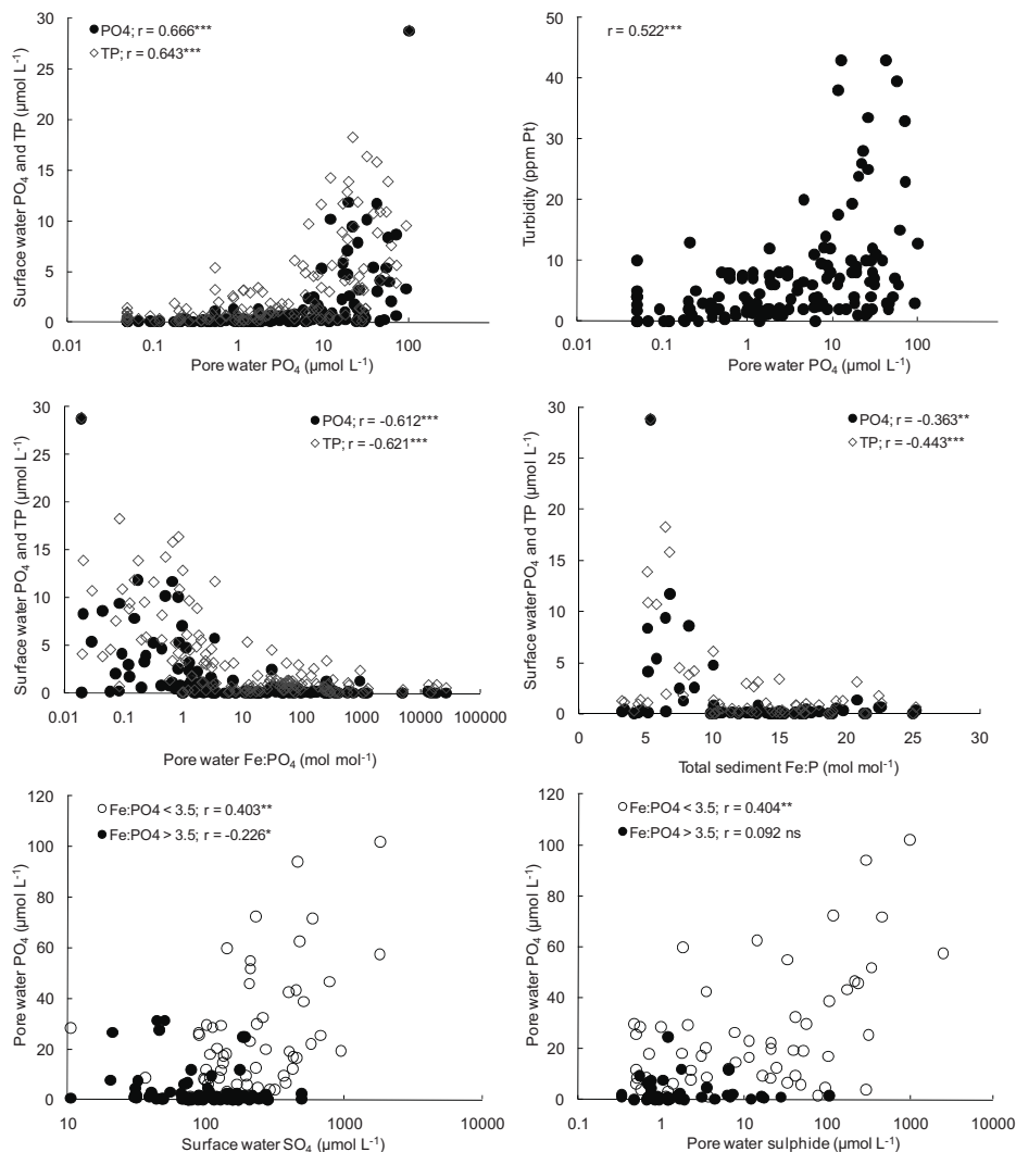
Figure 5. Relations between phosphate concentrations and other characteristics of pore water, surface water and sediment. Spearman's correlation coefficients are given. ns P > 0.05 , * P < 0.05 , ** P < 0.01 , *** P < 0.001 . Note the logarithmic x-axes, except for total sediment Fe:P.
