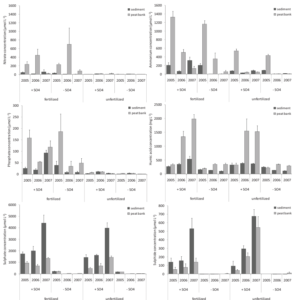
Figure 2. Effects of the various treatments on the pore water biogeochemistry of the peat bank and the sediment. Average concentrations (±SEM) are given for each year.
