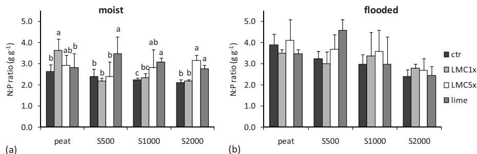
Figure 5. N:P ratios in plant tissue for the peat soil and the three sandy soil types under moist and flooded conditions after 243 days ( \pm SEM). Significant differences between treatments, as tested by univariate ANOVA ( P \leq 0.05 ), are indicated by different letters.
