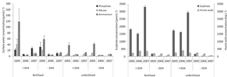
Figure 3. Effects of the various treatments on the surface water biogeochemistry. Average concentrations ( \pm\text{SEM} ) are given for each year.
