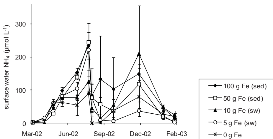
Figure 8. Effects of the various treatments on the NH 4 concentrations in the surface water ( \pm SEM). Treatments started after the second sampling date. Letters indicate differences between treatments ( P < 0.05 ). sw = surface water treatment, sed = sediment treatment.
