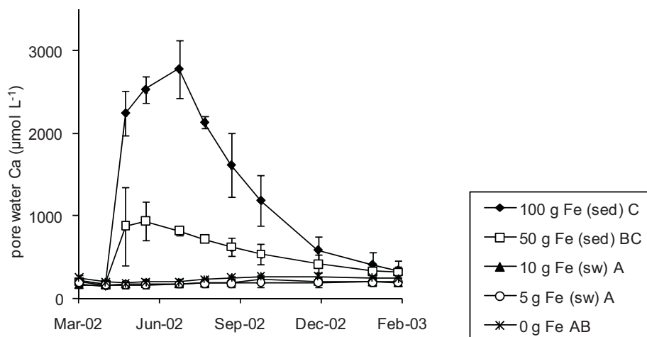
Figure 9. Effects of the various treatments on the Ca concentrations in the sediment pore water ( \pm SEM). Treatments started after the second sampling date. Letters indicate differences between treatments ( P < 0.05 ). sw = surface water treatment, sed = sediment treatment.
