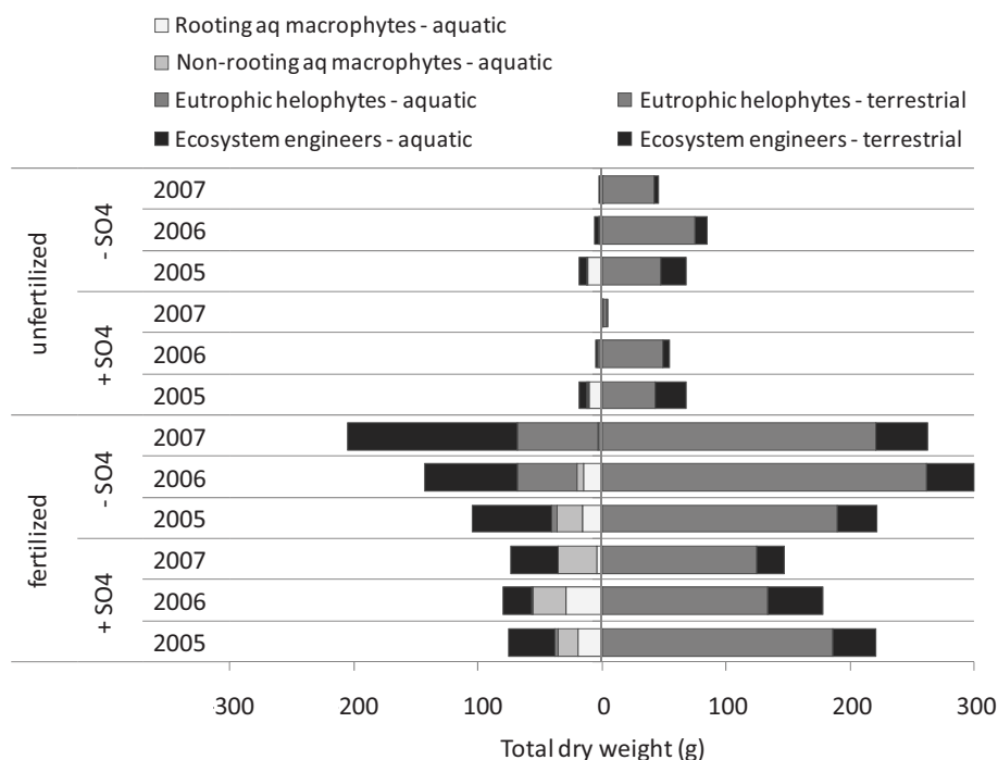
Figure 4. Effects of the various treatments on the biomass of rooting and non-rooting aquatic macrophytes, ecosystem engineers and eutrophic helophytes in the aquatic (left) and terrestrial (right) parts of the mesocosms. Starting biomasses for these plant groups were 5.2, 2.5, 17.5 and 4.4 g dry weight per mesocosm, respectively. Species are grouped as shown in Table 2.
