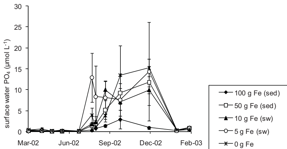
Figure 2. Effects of the various treatments on the \text{PO}_4 concentrations in the surface water ( \pm\text{SEM} ). Treatments started after the second sampling date. Letters indicate differences between treatments ( P < 0.05 ). sw = surface water treatment, sed = sediment treatment.
