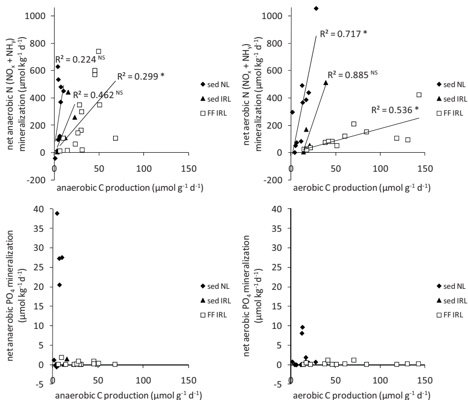
Figure 2. Relationship between C production rates and net mineralization rates of N ( \text{NO}_x and \text{NH}_4 ) and \text{PO}_4 during anaerobic (left) and aerobic (right) incubation in peat sediments (sed) and floating fen soils (FF) from different locations in the Netherlands (NL) and Ireland (IRL). The relations between C production and net N mineralization rates were described by linear regression analysis (* P < 0.05 , NS P > 0.05 ).
