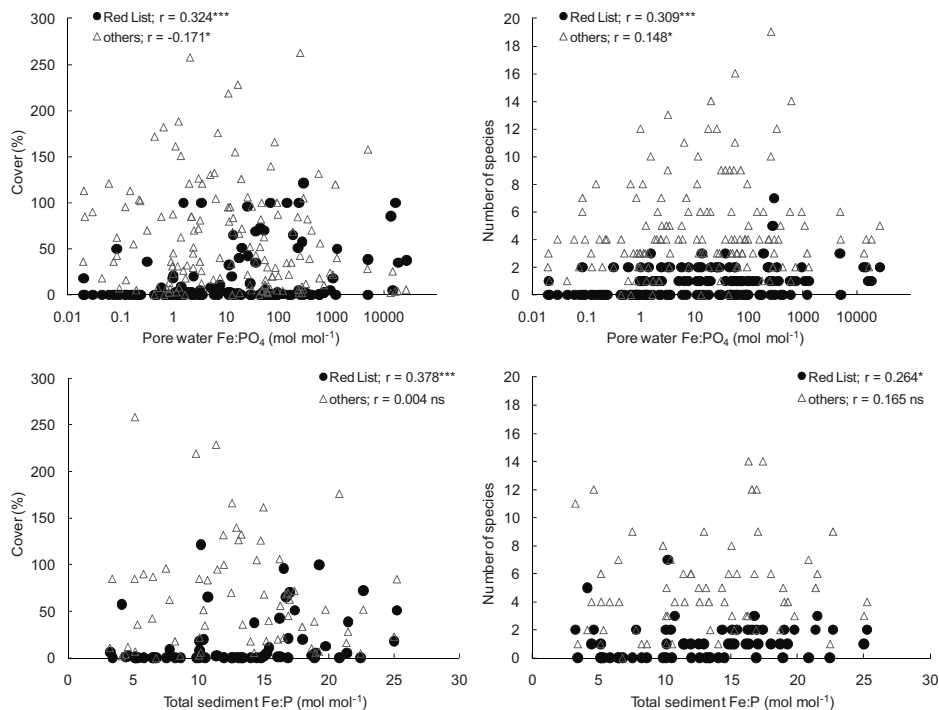
Figure 6. Percentage cover and number of macrophytes, divided into Red List species and others, plotted against pore water Fe:PO 4 and sediment Fe:P ratios. Spearman's correlation coefficients are given. ns P > 0.05 , * P < 0.05 , ** P < 0.01 , *** P < 0.001 . Note the logarithmic x-axes for pore water Fe:PO 4 .
